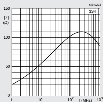
Impedance as a function of frequency.
